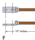
Single-Lug Bond Stub with 2-Hole NEMA Lug (Straight)
