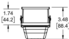
Adapter, Duplex Insert, Plastic, 1-Gang
