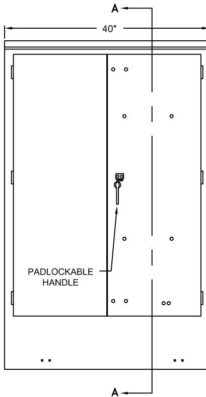
FRONT ELEVATION ENCLOSED
