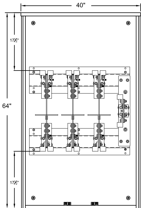
FRONT ELEVATION LESS FRONTS
