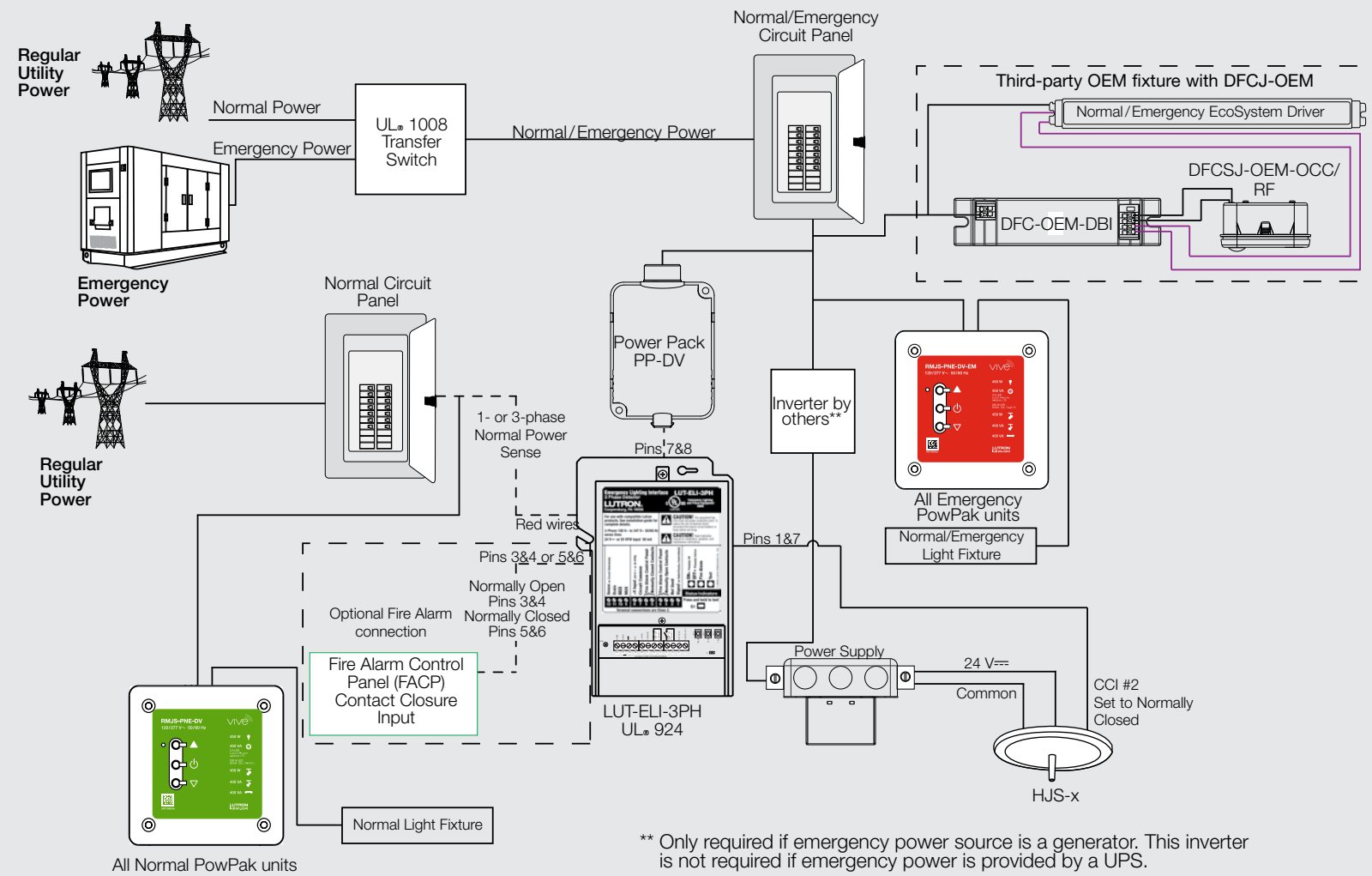
System Wiring Diagram (Vive hub with 347V emergency dimming module)
