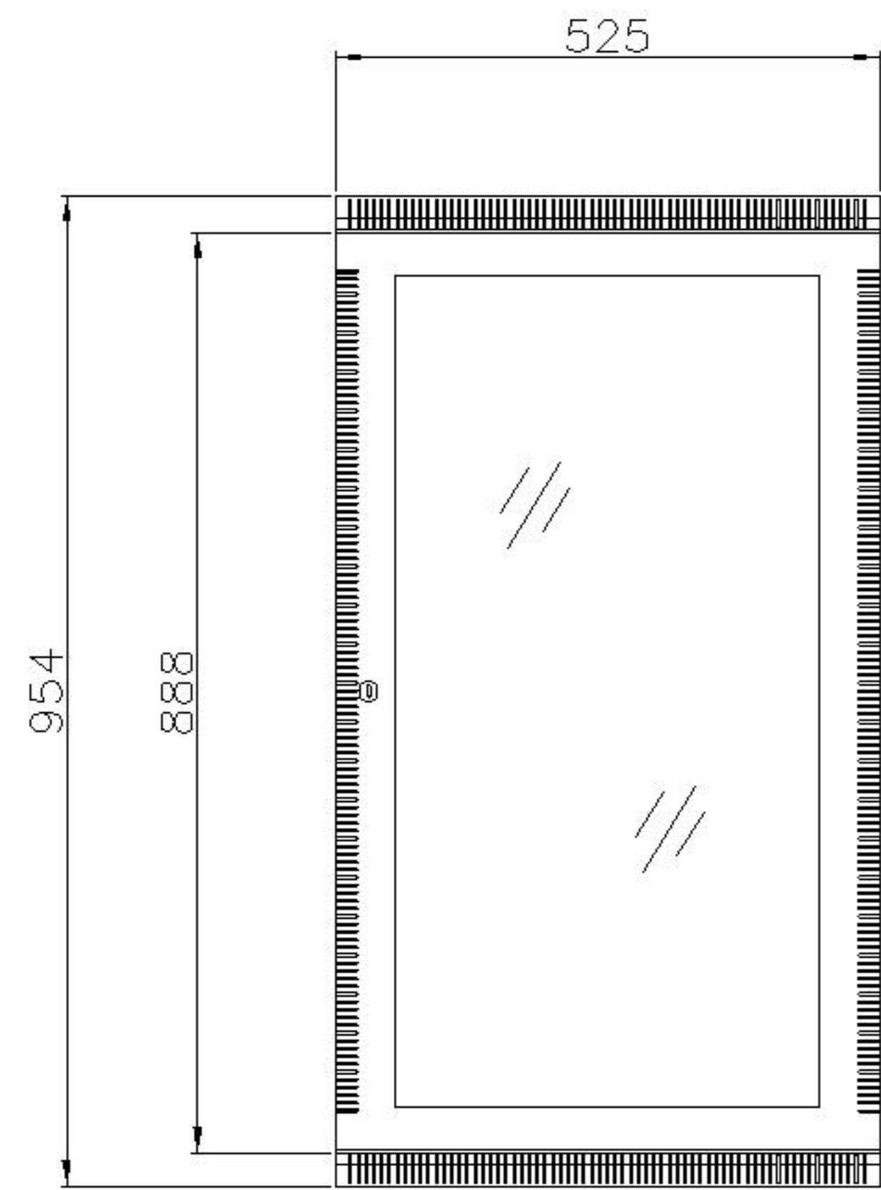
Front
