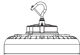
65-771R2: \varnothing 13.4" (340±5mm)
