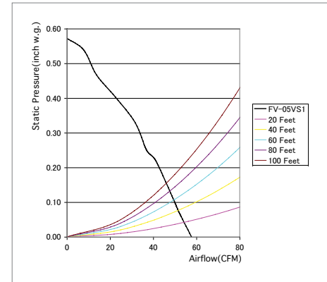
FV-05VS1 50 CFM 4" Oval Duct
