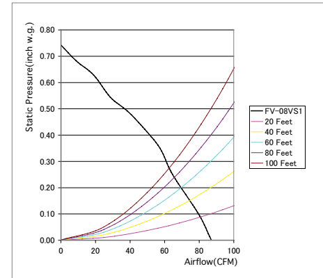
FV-08VS1 80 CFM 4" Oval Duct
