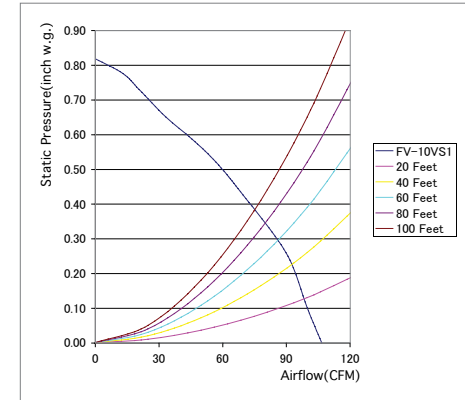
FV-10VS1 100 CFM 4" Oval Duct
