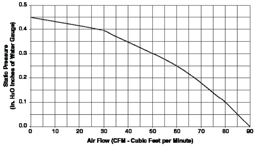
Model AEN80B
