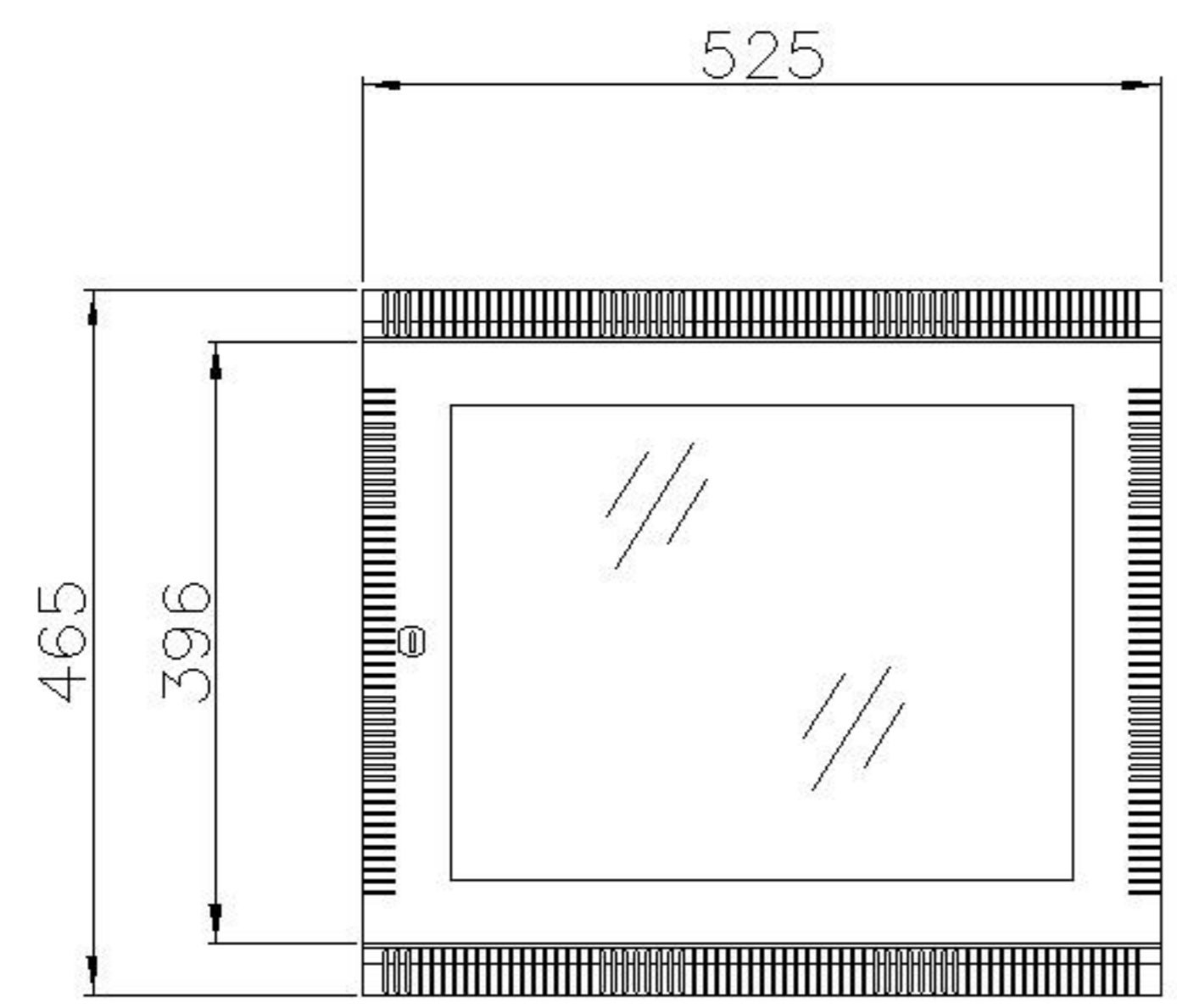
Front
