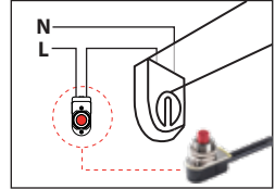
3. Connect Emergency Test Switch
