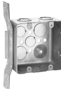
"VS" bracket
