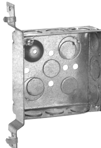
"VP" bracket
