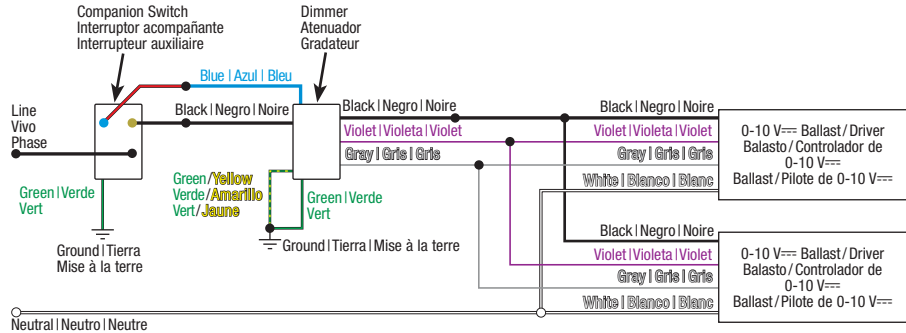
Image #62 — Dimmer with Two Black Wires, One Blue Wire, One Violet Wire and One Gray Wire in a 3-Way Application with a Companion Switch
