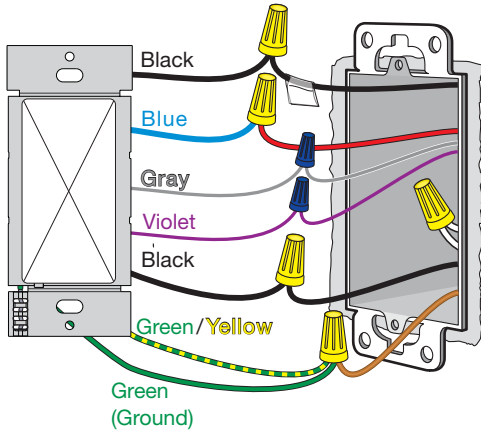
Image #62 — Dimmer with Two Black Wires, One Blue Wire, One Violet Wire and One Gray Wire in a 3-Way Application with a Companion Switch
